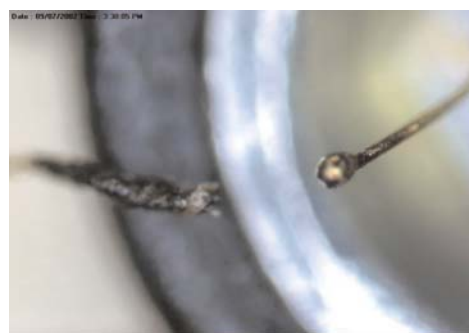
Figure 17. Fused wire failure.
